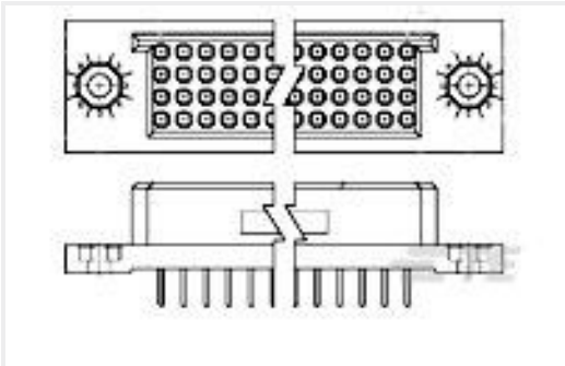
TE Part #533285-5 BOX II 4 ROW RECP ASSY 160 POS
