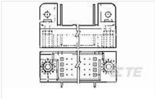
TE Part #533286-5 HDI PIN ASSY 4 ROW 160 POS R/A
