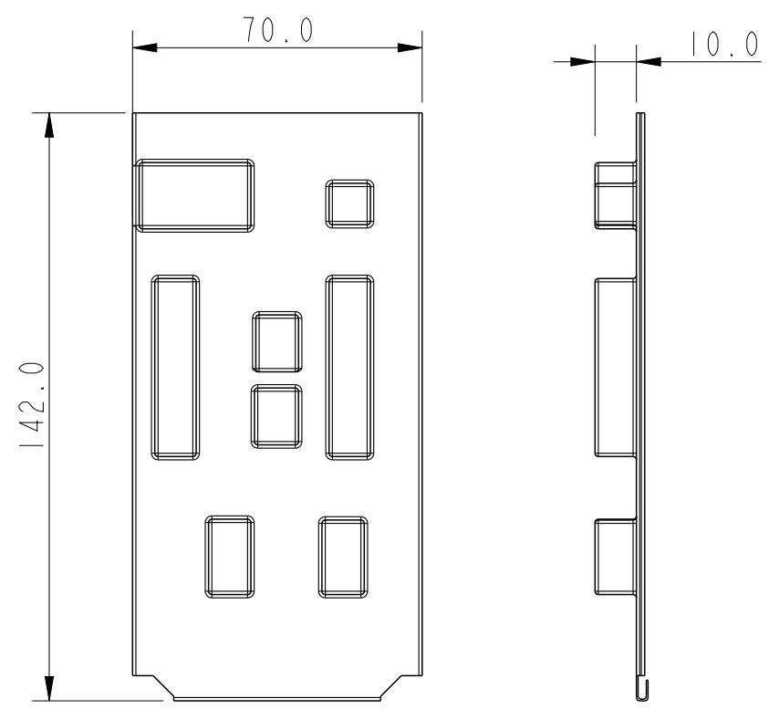
BLISTER PACKING WITH ASSEMBLY INSTRUCTION CARD
