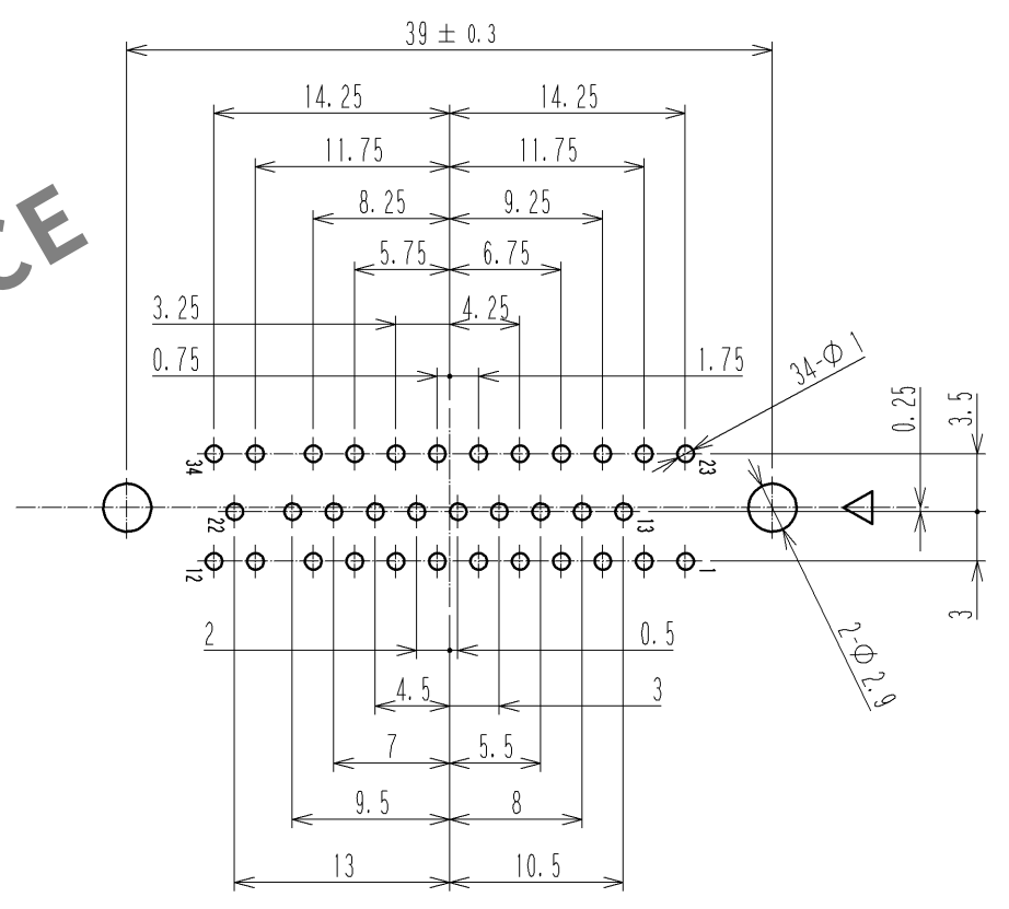
RECOMMENDED PC BOARD PATTERN
