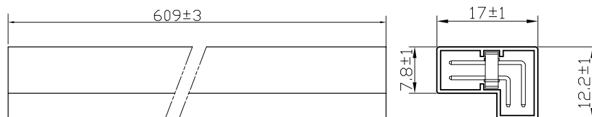
TUBE PACKAGE
