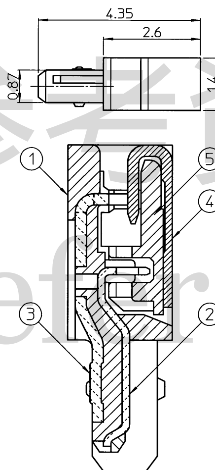
X-X' Cross-section(20:1)
