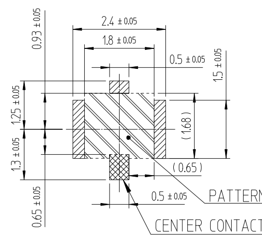
RECOMMENDED PCB/METAL MASK PATTERN DRAWING(5:1)
