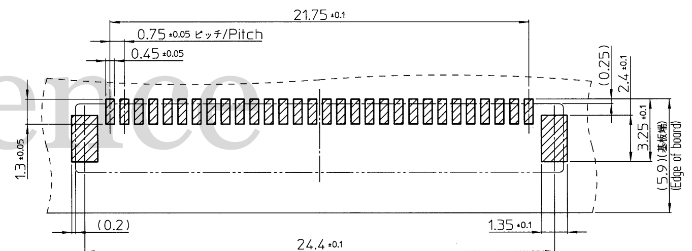
参考基板設計要領(コネクタ搭載面) Reference Board Design Procedure (Connector Mounting Surface)
