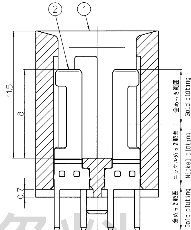
X-X'断面(5:1) X-X' Cross-section(5:1)
