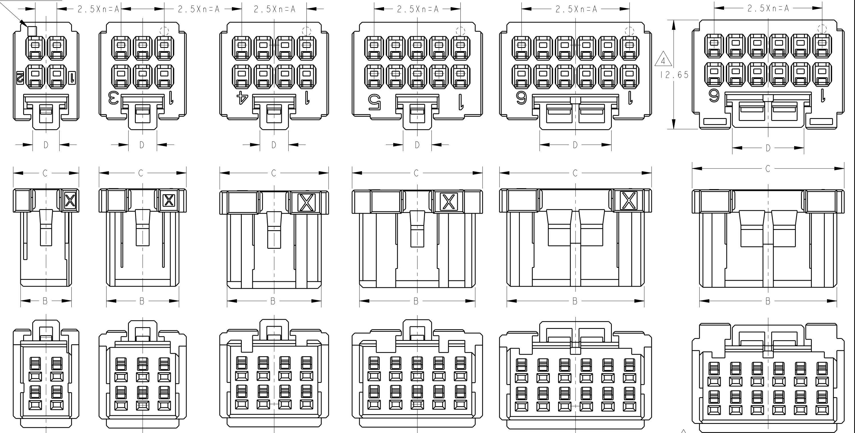
10POS(X-KEY): 1-1827864-5 12POS(X-KEY): 1-1827864-6
