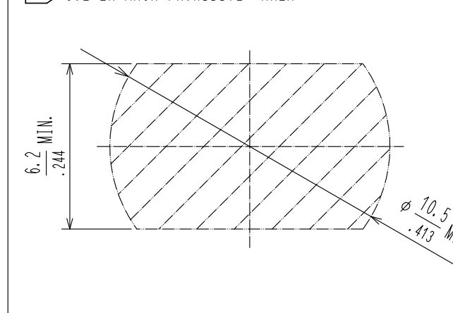
4 SOLDER MASK PROHIBITED AREA
