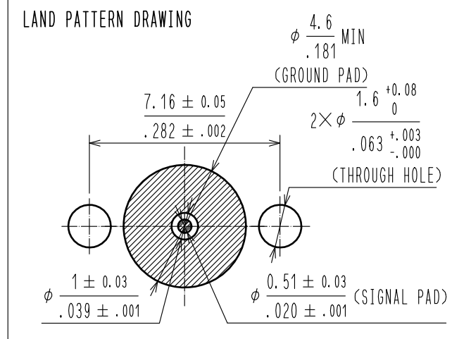
4 SOLDER MASK PROHIBITED AREA
