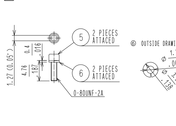
3 DRAWING OF SOCKET HEAD CAP SCREW (2:1)
