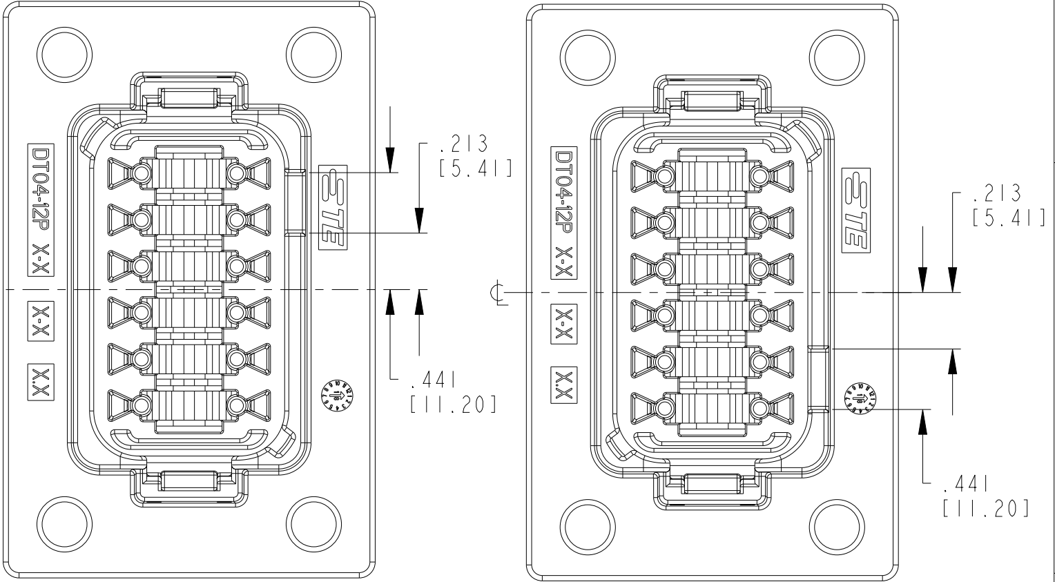
KEY ARRANGEMENT -D- DT04-12PD-BL12
