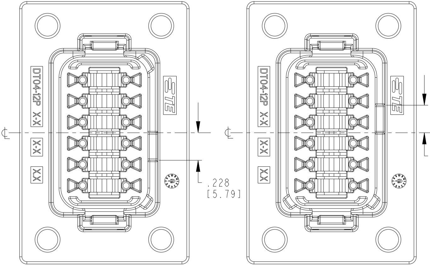
KEY ARRANGEMENT -A- DT04-12PA-BL12
