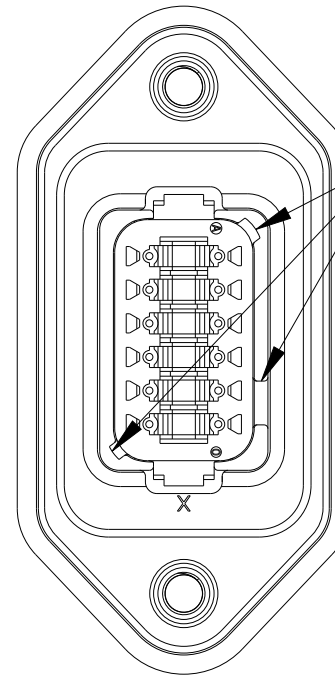
DT04-12PD-LE21 KEY ARR. -D- HOUSING COLOR: BROWN
