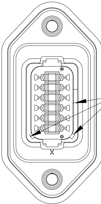
DT04-12PB-LE21 KEY ARR. -B- HOUSING COLOR: BLACK
