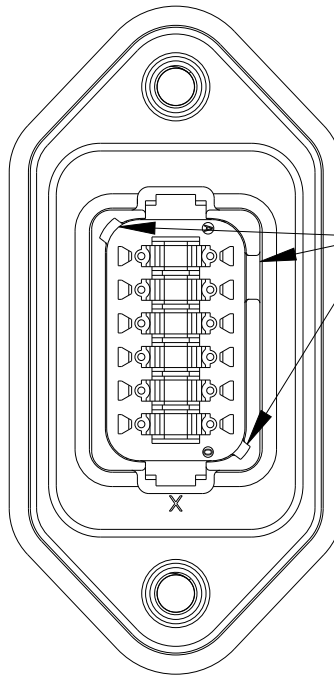
DT04-12PC-LE21 KEY ARR. -C- HOUSING COLOR: GREEN
