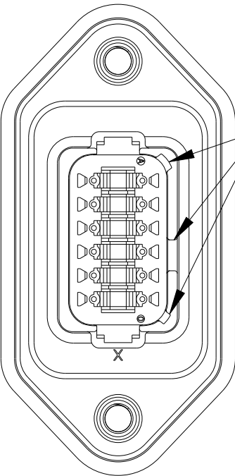
DT04-12PA-LE21 KEY ARR. -A- HOUSING COLOR: GRAY
