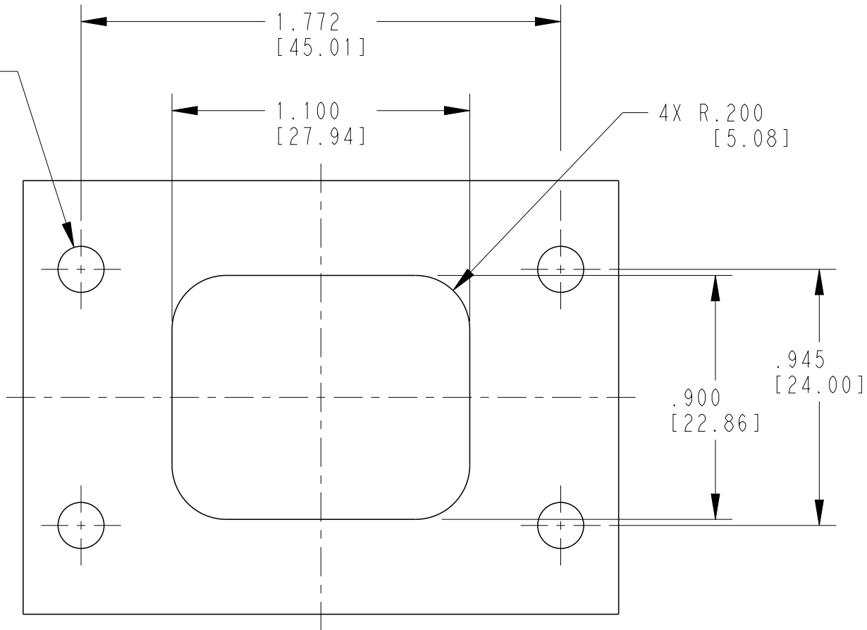
RECOMENDED PANEL CUTOUT REAR
