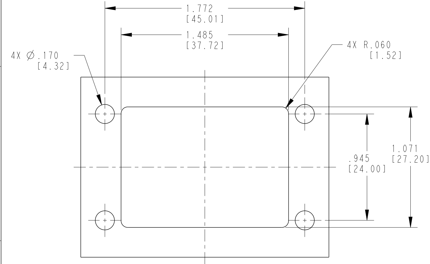
RECOMENDED PANEL CUTOUT FRONT
