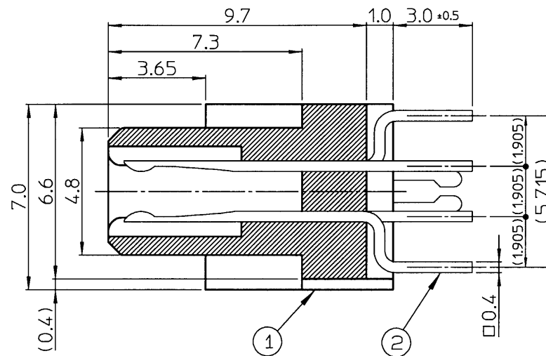
X-X' Cross-section(Scale 5:1)
