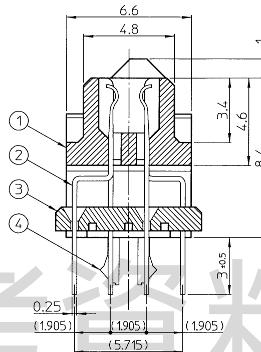
X-X' Cross-section (Scale 5:1) X-X'断面(5:1)
