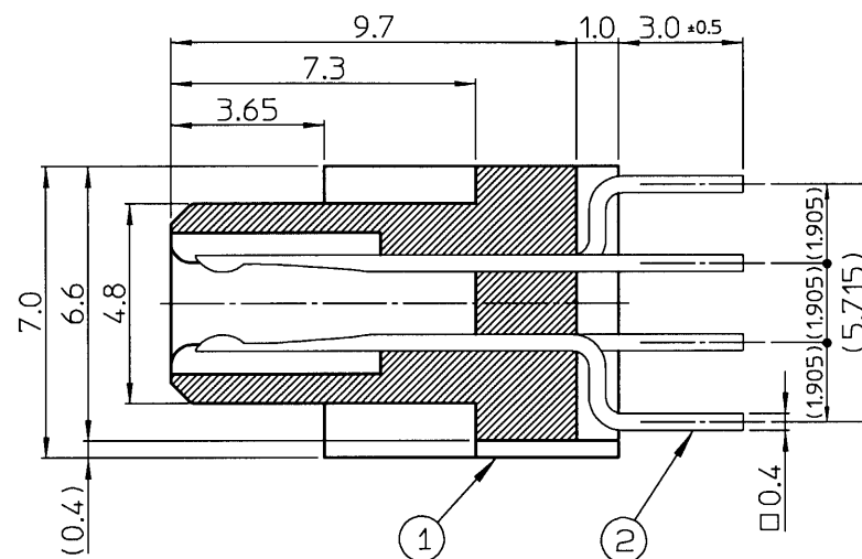
X-X' Cross-section(Scale 5:1)
