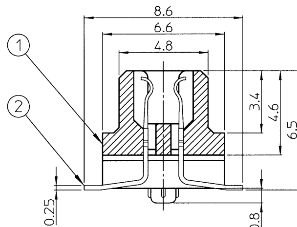
X-X' Cross-section (Scale 5:1) X-X' 断面 (5:1)
