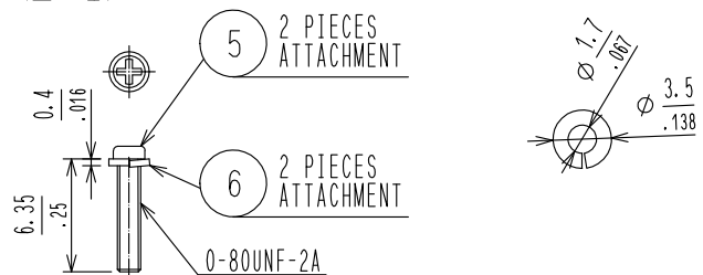
(2 : 1) PART⑥ OUTLINE DRAWING
