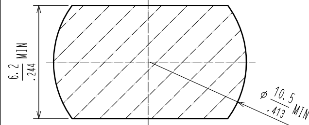
4 SOLDER MASK PROHIBITED AREA
