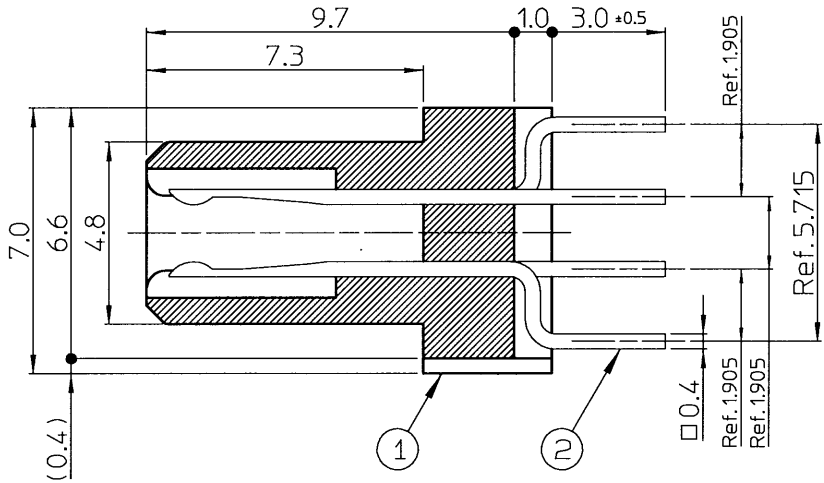
X-X' Cross-section(Scale 5:1)
