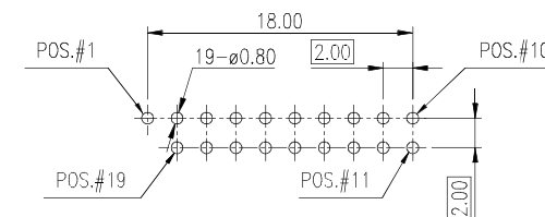
RECOMMENDED PCB LAYOUT (TOP VIEW) (ALL TOLERANCES ARE ±0.05)
