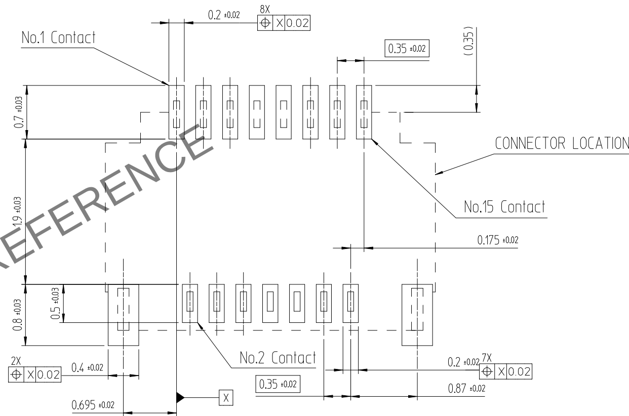
RECOMMENDED PCB PATTERN (RECOMMENDED METAL MASK = 0.1mm) (SCALE FREE)
