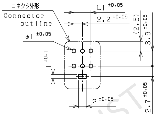
6P推奨基板穴寸法 (コネクタ装着側) 6P Recommendable P.C. Board hole layout (connector mounted side)
