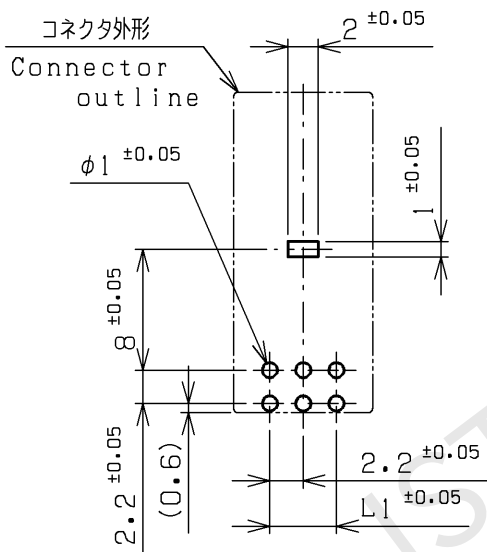
6P、8P推奨基板寸法 (コネクタ装着側) 6P、8P Recommendable P.C. Board hole layout (connector mounted side)
