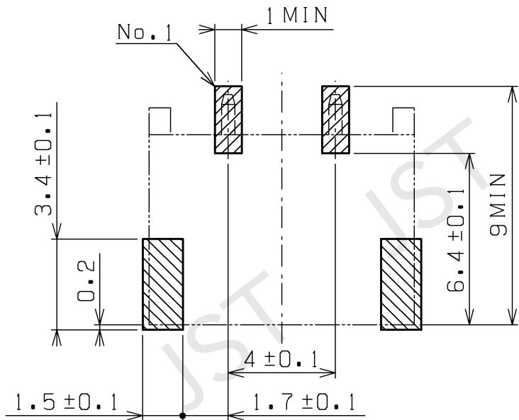
推奨基板レイアウト (部品上面側) Recommendable P.C.Board layout (From top view)
