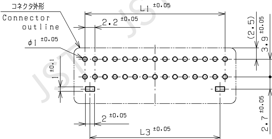
推奨基板寸法 (コネクタ装着側) Recommendable P.C. Board hole layout (connector mounted side)
