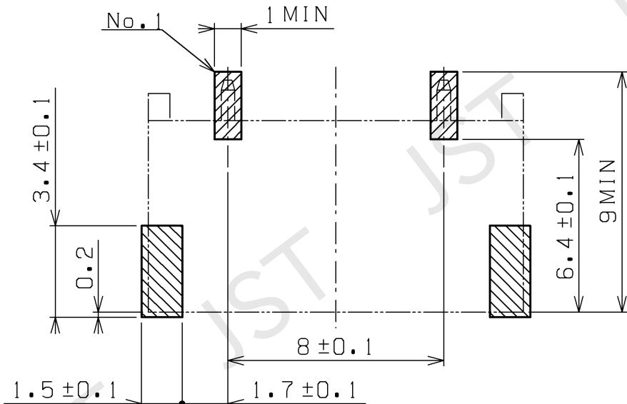
推奨基板レイアウト (部品上面側) Recommendable P.C.Board Layout (From top view)
