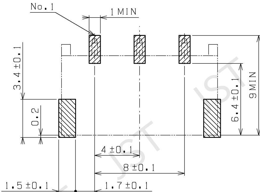
推奨基板レイアウト (部品上面側) Recommendable P.C.Board layout (From top view)
