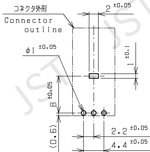
推奨基板穴寸法 (コネクタ装着側) Recommendable P.C. Board hole layout (connector mounted side)
