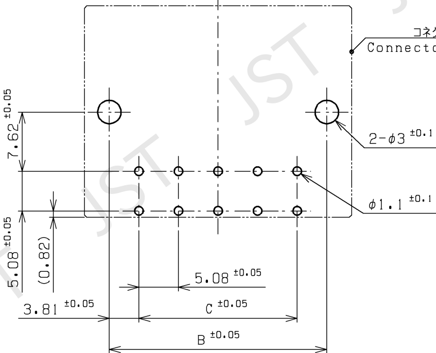
推奨基板穴寸法 (コネクタ装着側) Recommendable P.C. Board hole layout (connector mounted side)
