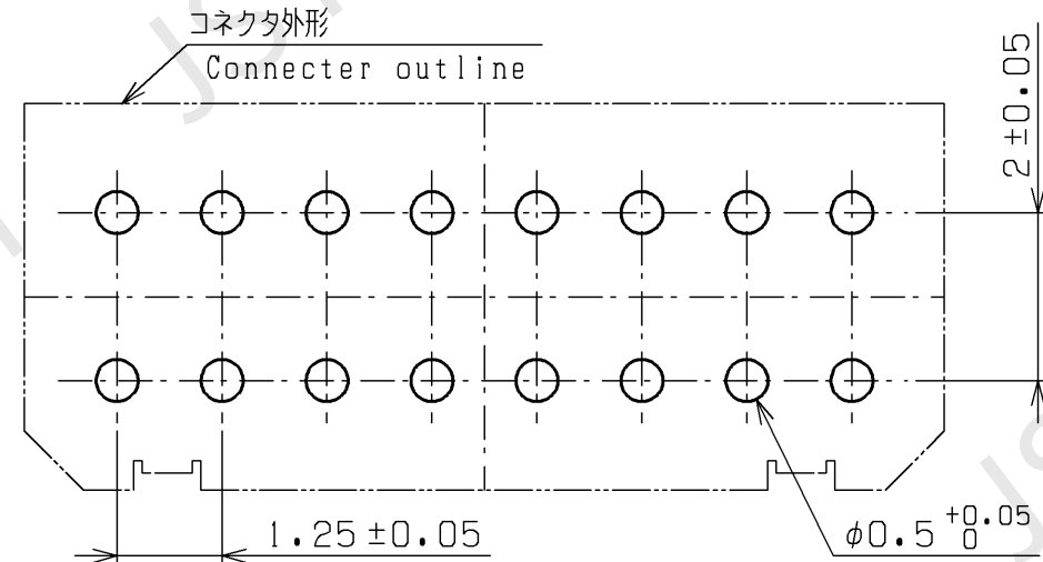
推奨基板穴寸法(コネクタ装着側から見た図) Recommendable P.C.Board hole layout (The figure viewed from connector mounting side.)
