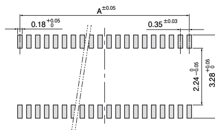
Recommended metal mask layout
