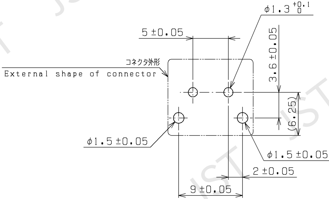
推奨基板穴寸法 Recommendable P.C.Board hole layout
