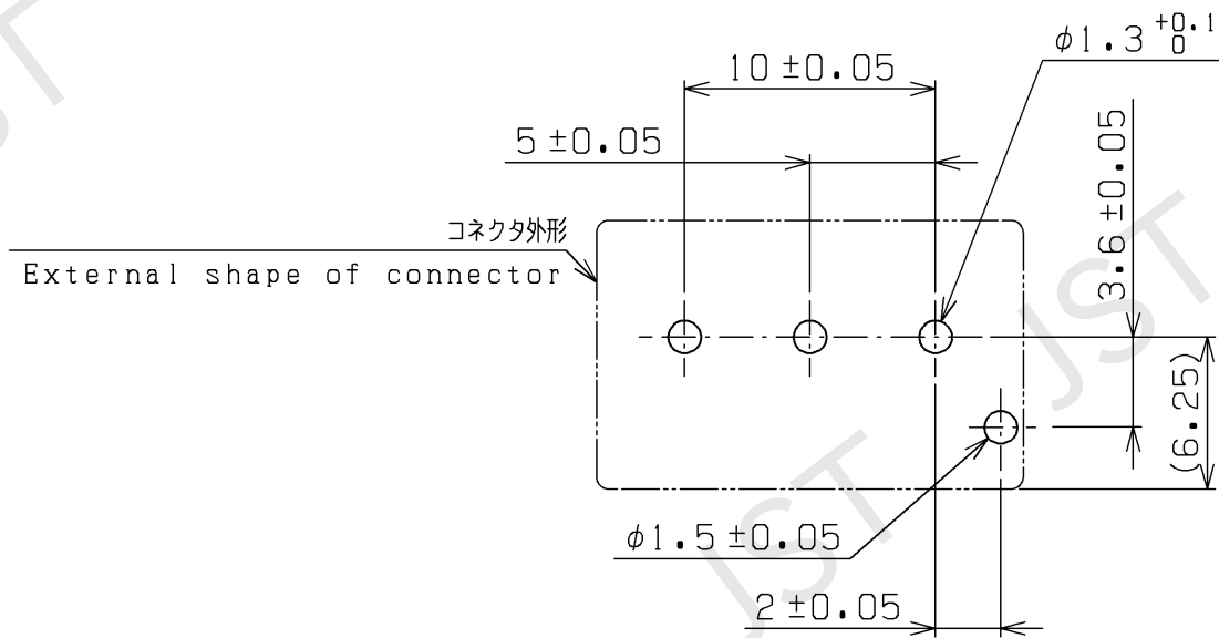
推奨基板穴寸法 Recommendable P.C.Board hole layout
